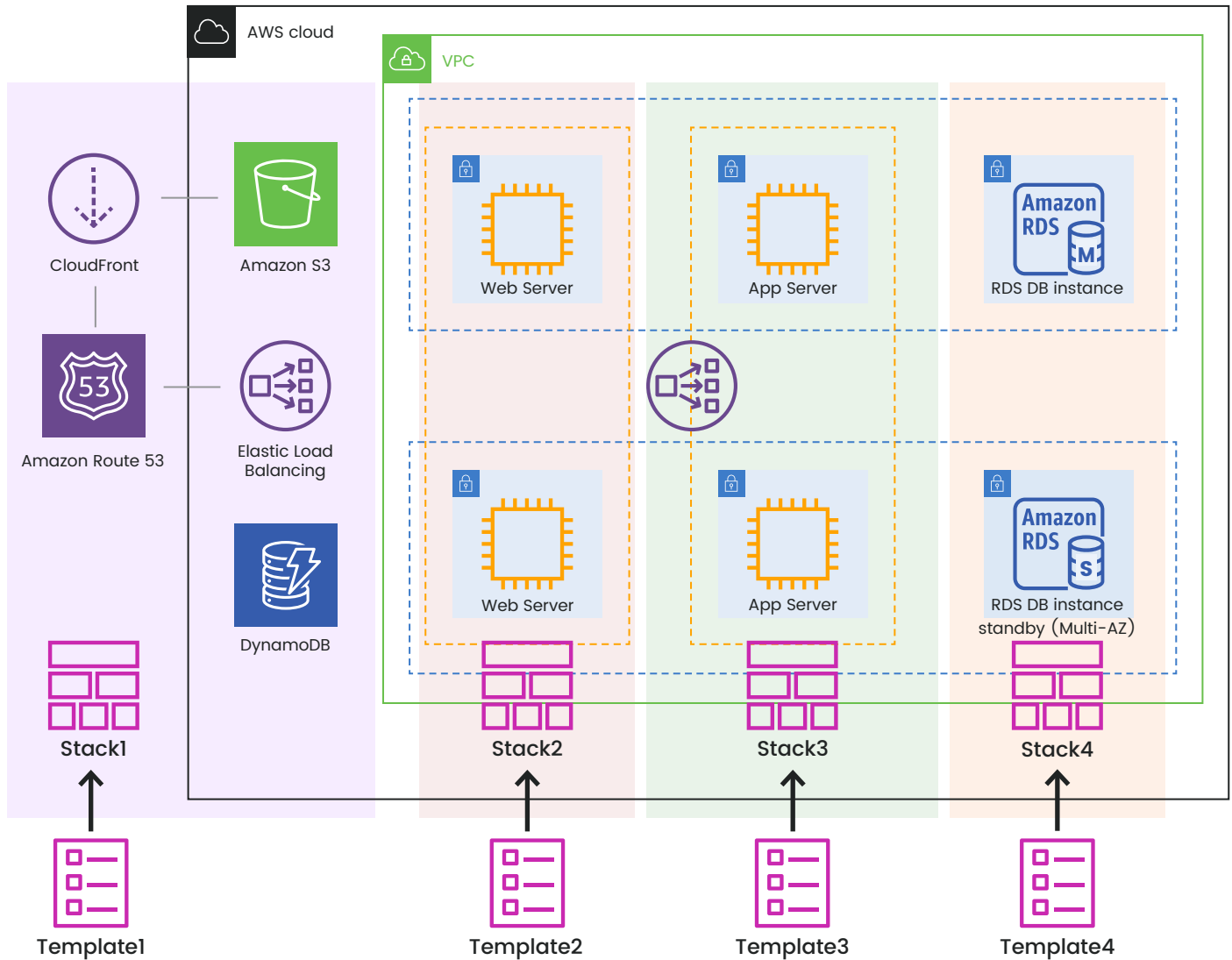
Figure 4: AWS CloudFormation example 2 – creating an entire environment (stacks) from multiple templates in a layered approach
